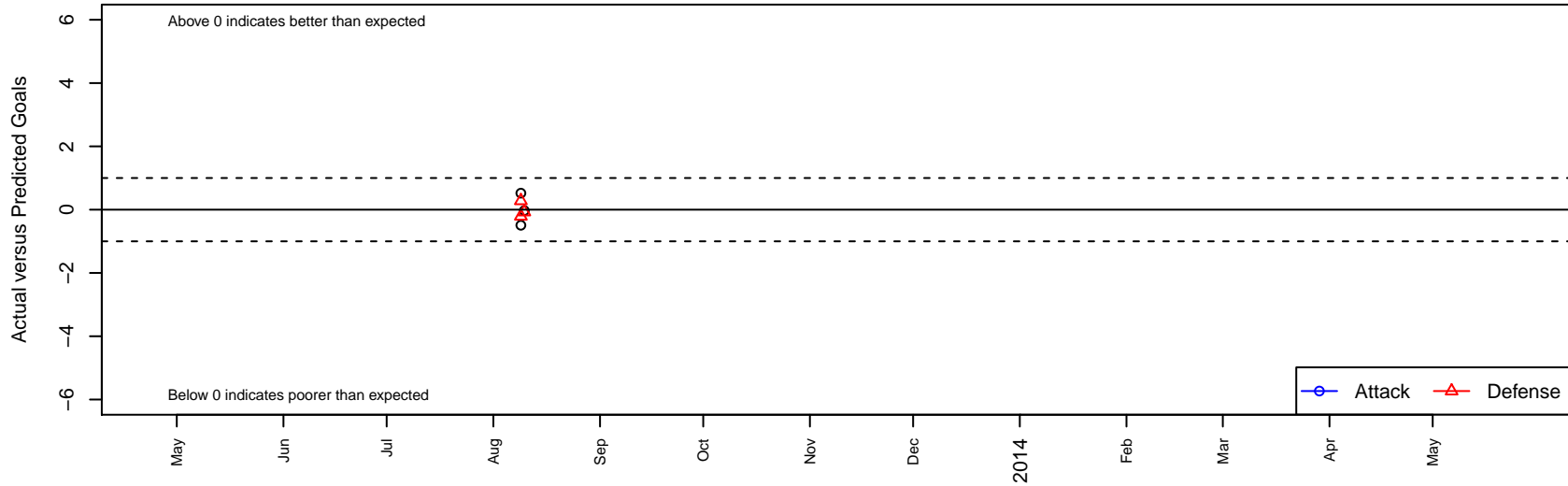
MVLA Avalanche Blue G01 Dots are actual minus expected GF (blue circles) and GA (red triangles). Blue line is smoothed change in attack strength. Red is smoothed change in defense strength.
